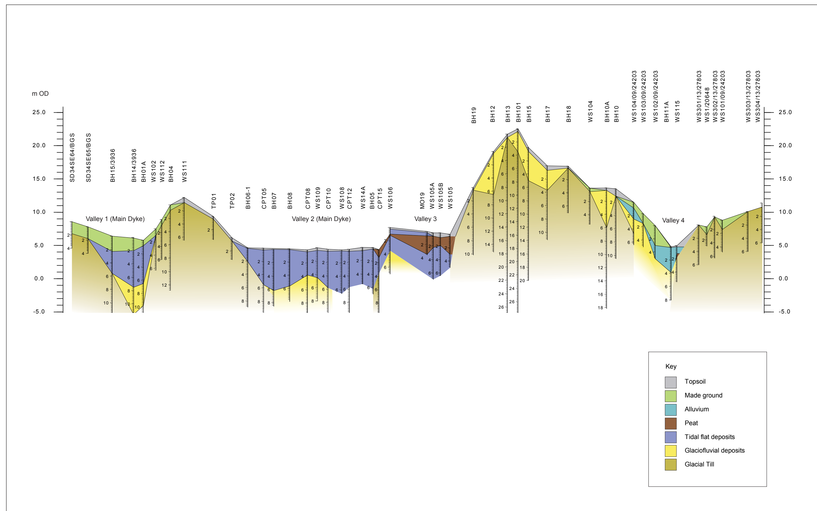
Figure 3: Stratigraphic transect
